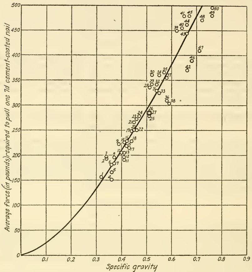
FIGURE 15.—Relation of specific gravity of wood to nail-holding power; sevenpenny cement-coated nails driven 1¼ inches into side grain and pulled at once
